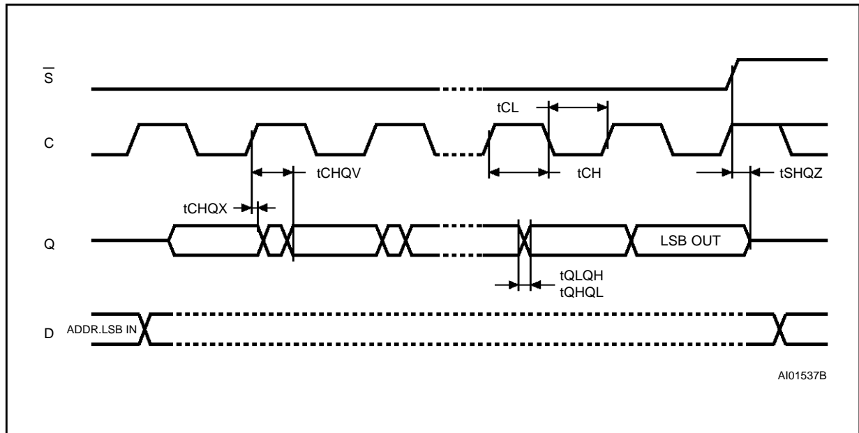
Figure 16. Output Timing
